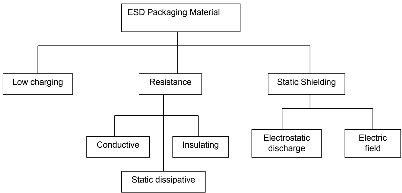
Figure 1: Classification of materials for ESD protection
